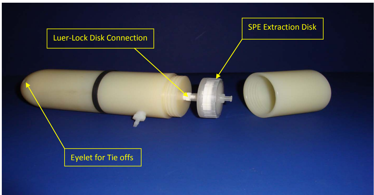
Partially Assembled unit
